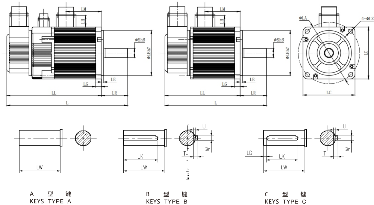
尺寸图 DIMENSIONAL DRAWING
