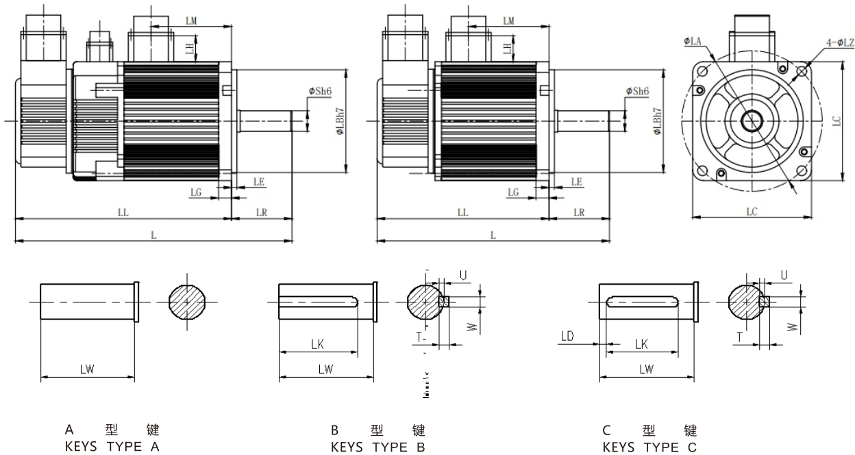
尺寸图 DIMENSIONAL DRAWING
