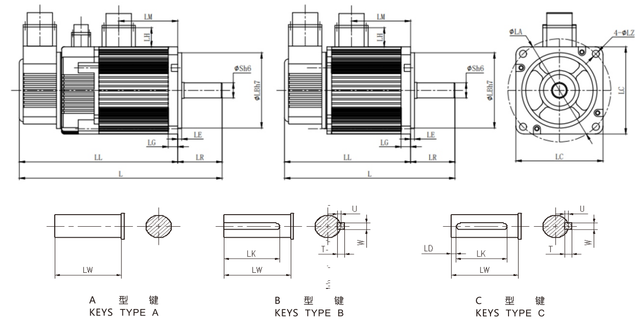
尺寸图 DIMENSIONAL DRAWING
